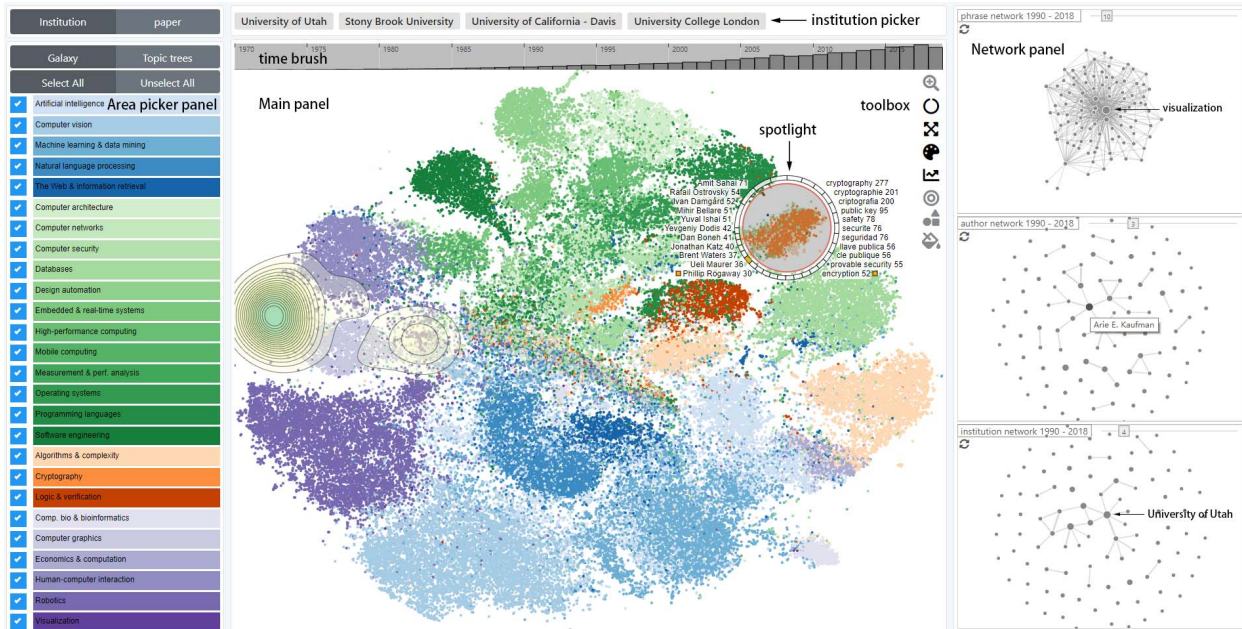
Fig. 1: Interface of Galex consists of three panels: area picker panel (left), main panel (middle), and network panel (right). The main panel includes three layers: discipline, area, and institution layers. To date, all papers (over 86,000) from all 26 areas are shown in the discipline layer, forming an overview (galaxy) of computer science. The area picker controls the areas that are displayed. A contour line indicates the paper distribution of one area (here, visualization). The spotlight reveals the semantics of the regions of interest. The time brush acts as a time filter. The toolbox provides useful components, such as pallet, spotlight, and time slice selector. The network panel includes three kinds of networks to uncover the structure of one area.
